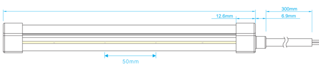
Side view
