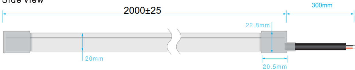
Side view
